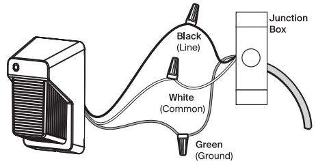
Wiring Diagram
